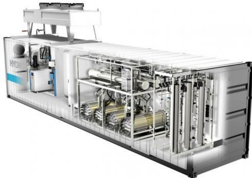
Figure 35. Sketch of Hydrogenics electrolyzer skid.
