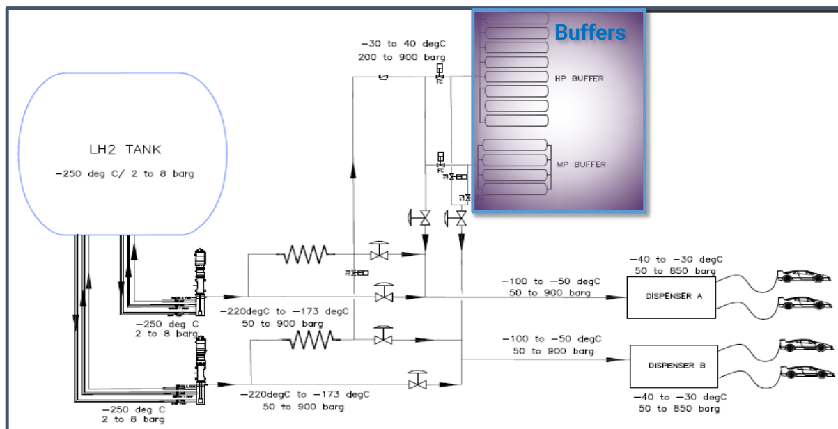
Figure 25. Process flow of a LH2-based refuelling station – Gaseous buffers.
