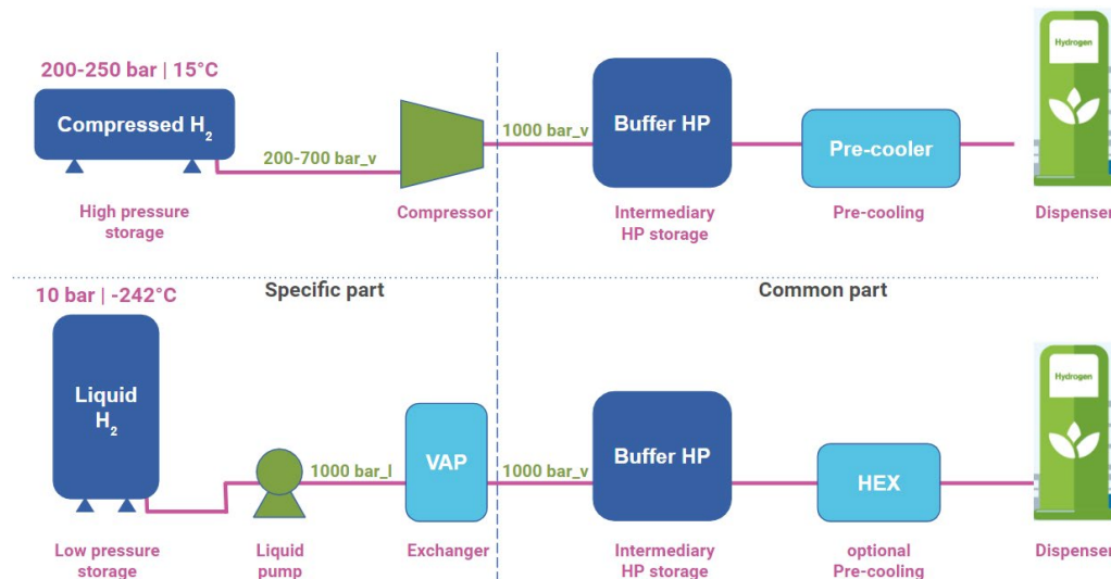
Figure 8. Simplified comparison between gaseous and liquid hydrogen refuelling stations. Top: gaseous HRS, bottom liquid HRS.
