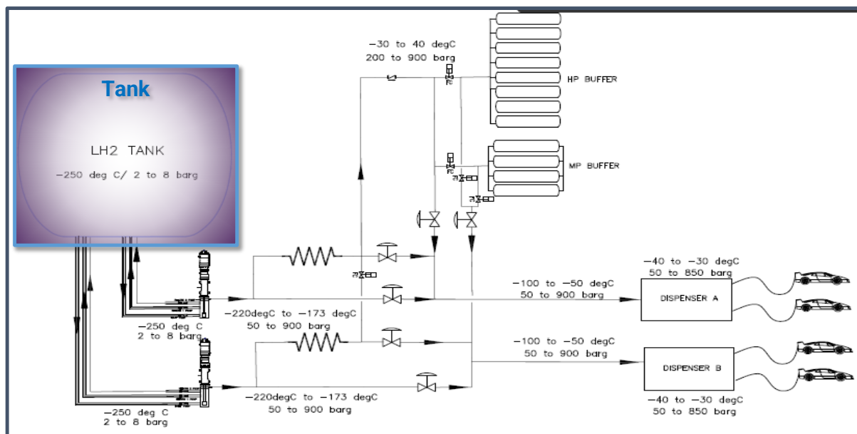
Figure 15. Process flow of a LH 2 -based refuelling station – LH 2 storage tank
