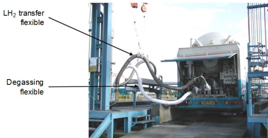
Figure 38. LH 2 trailer during transfer.
