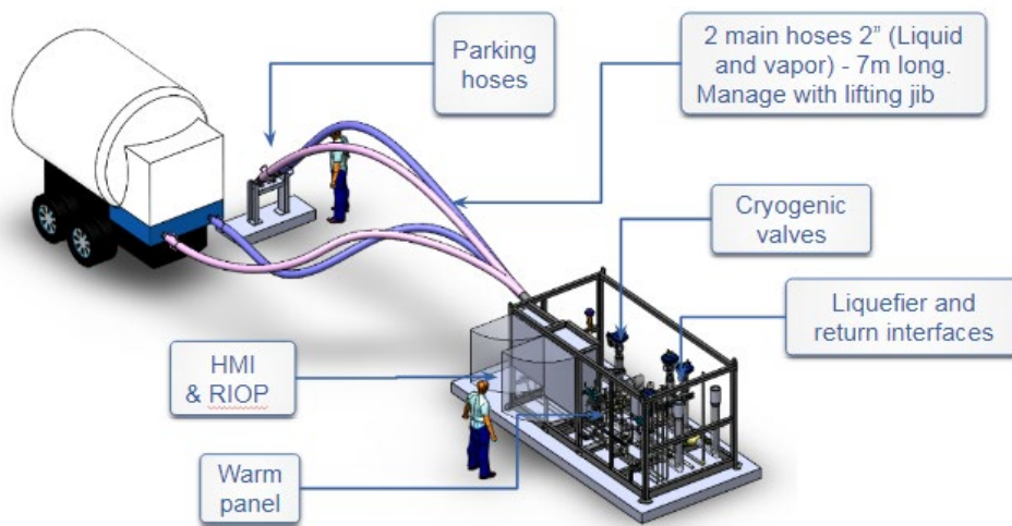
Figure 37. Generic loading bay ergonomics for LH 2 trailer filling.
