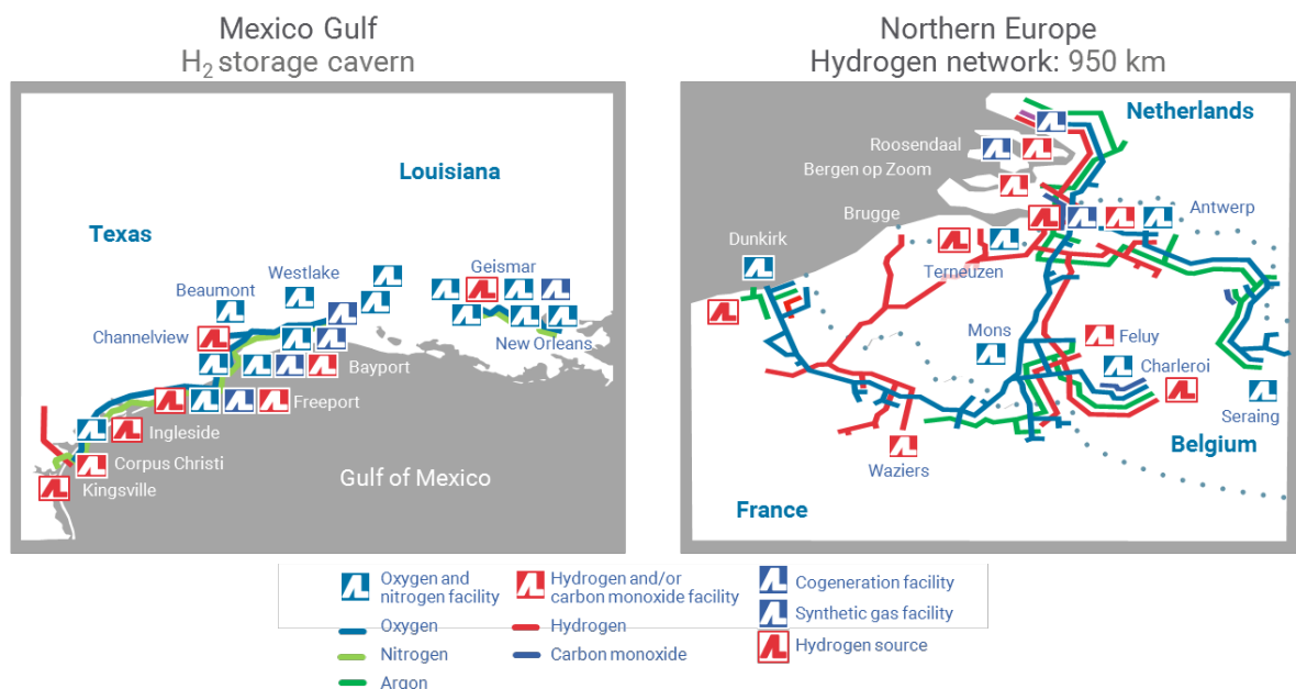
Figure 39. Air Liquide hydrogen sources and network.
