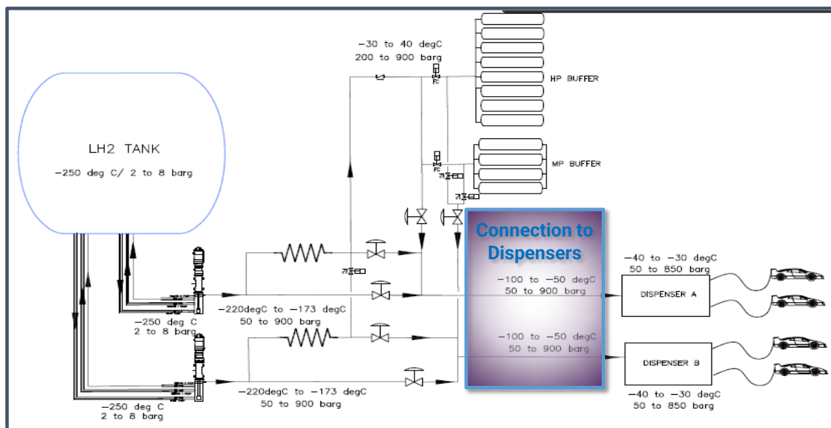
Figure 27. Process flow of a LH 2 -based refuelling station – Connection to dispenser(s).
