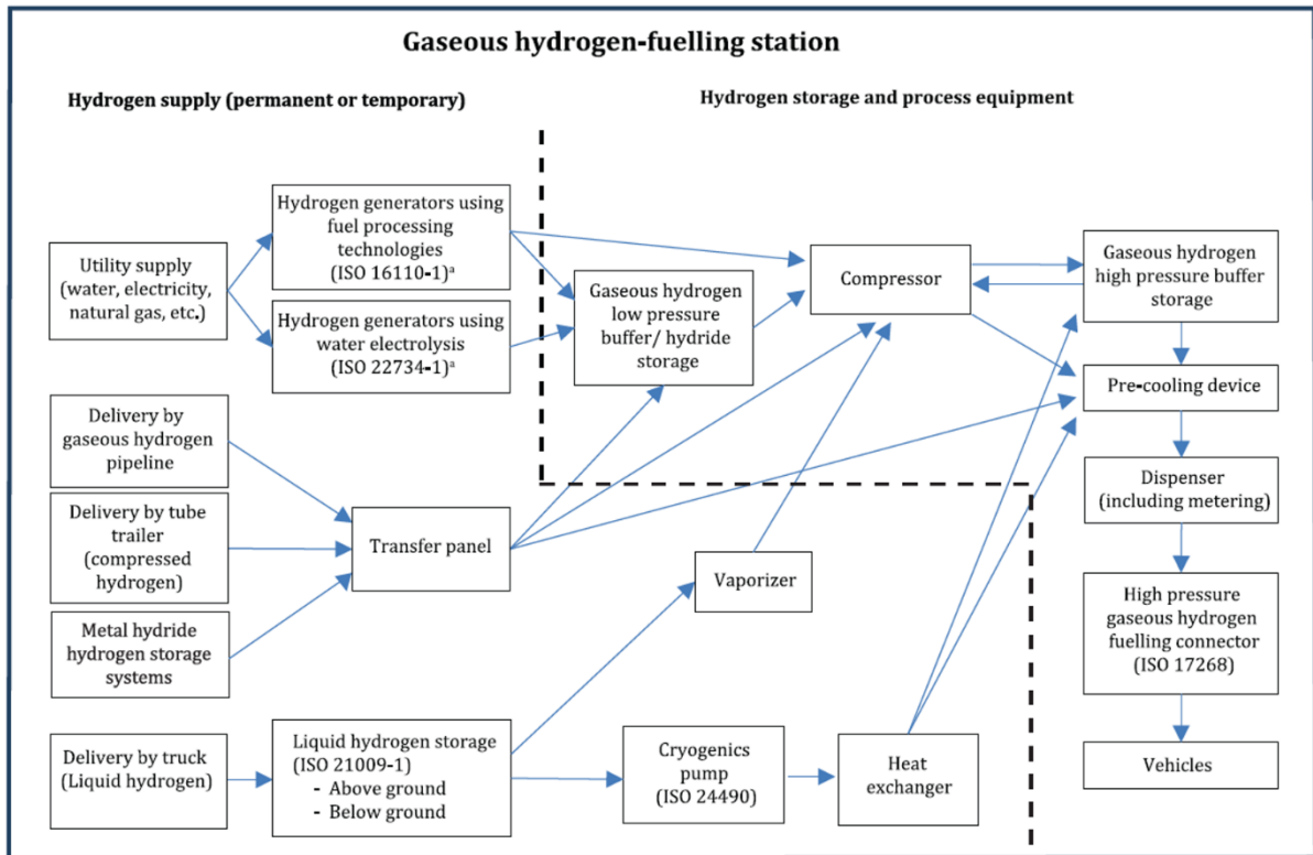
Figure 4. Example of typical elements of a fuelling station including hydrogen supply [2]
