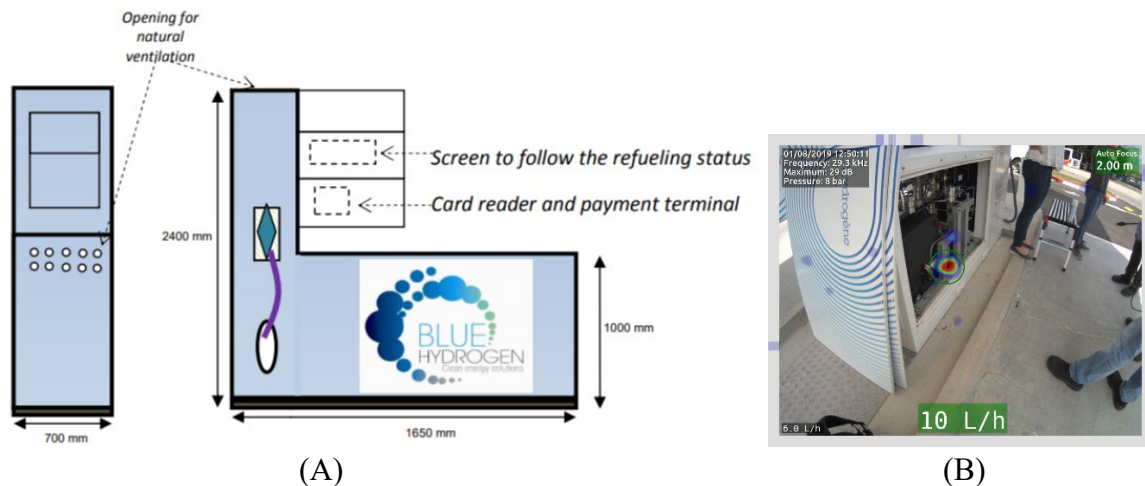
Figure 28. (A) Dispenser main elements and indicative dimensions, (B) valve skid.
