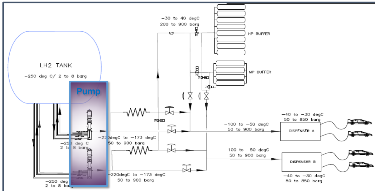
Figure 18. Process flow of a LH 2 -based refuelling station – LH 2 pump.
