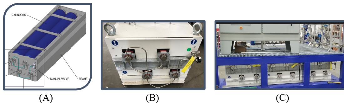
Figure 26. High pressure buffers. (A) 4 type-II buffers in a bundle, (B) Interconnections at buffer heads, (C) Integration of bundles in the LHRS skid.
